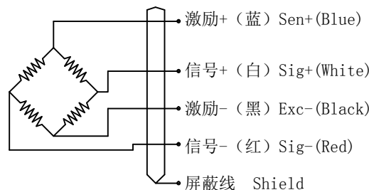
接线图Wiring Schematic Diagram
